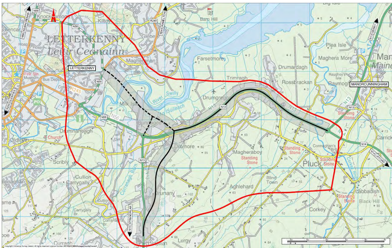
Figure 17-2 Section 2 Preferred Option
